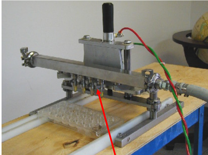
Nozzle configuration Indexes down to deposit and up to break thread
