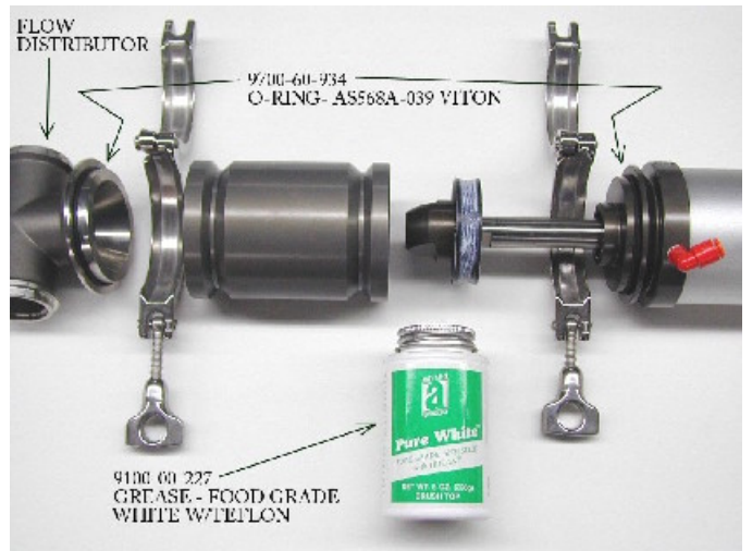
Partial exploded view of depositing pump Easily disassembled for cleaning!
