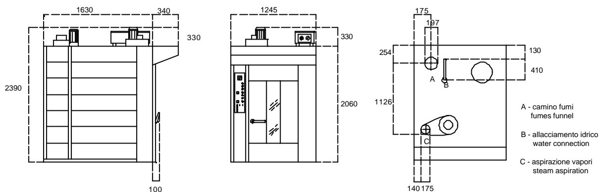
ROTOR mod. 57
