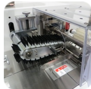
Upper Brush Pushes Air Out of the Bag
