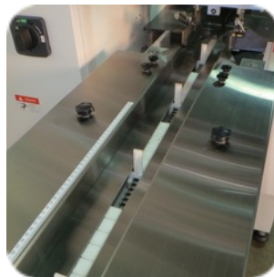
7ft. Flighted Infeed with Product Carriers
