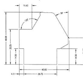
SIDE VIEW Service Case
