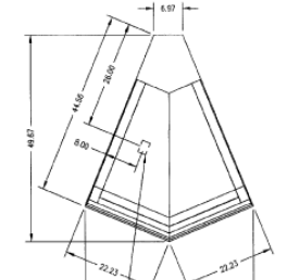
TOP VIEW SQROC45SSR
